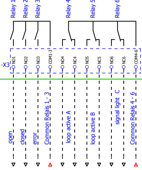
Relay Outputs
