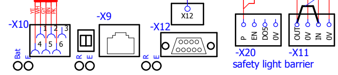
barrier controller MGC
